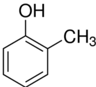
O-cresol
