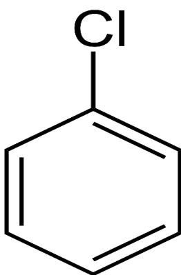
o-cloromobencenoh
